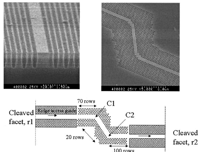
FIG. 1. Cross and top view micrographs of W2-PC guide; schematic of the structure measured.
